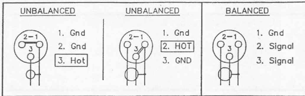
Fig. 6-0: Audio Connections
